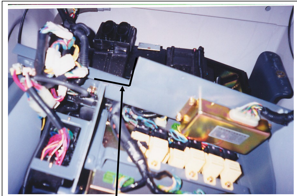
Notch out extra metal on back of computer frame to make room for flex ducts before reinstalling
