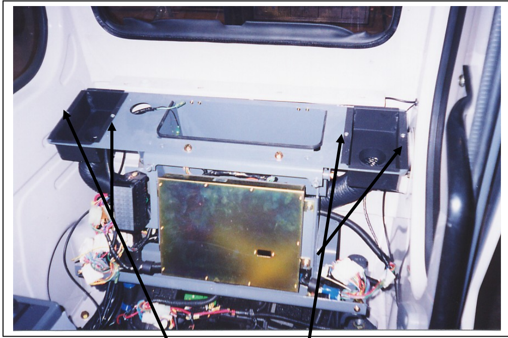
Secure the air boxes with the self drilling screws provided
