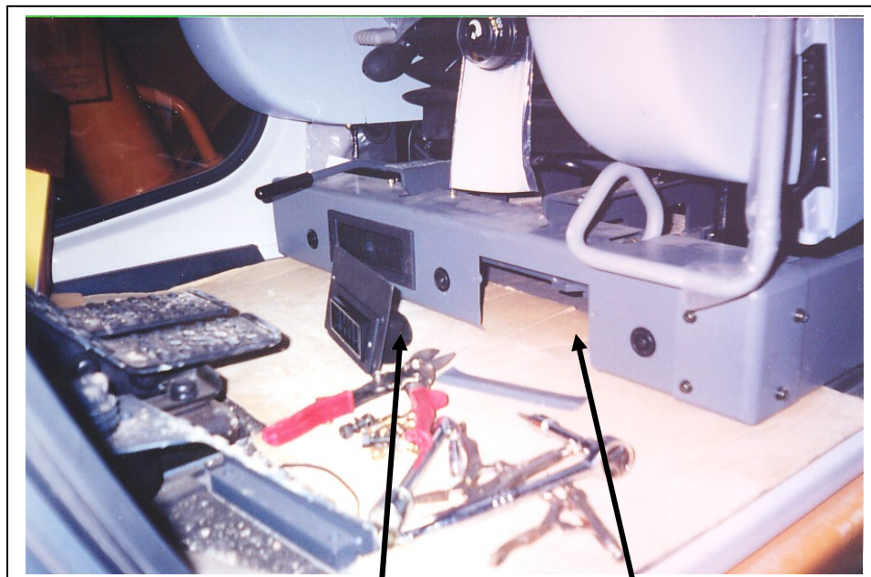
New louver assembly
