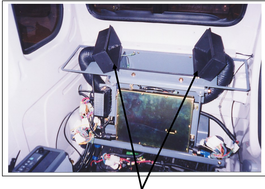
Rear louver air boxes connected to flex duct ready to install in large rectangular holes
